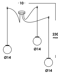
10/s3 dec. 3 G9 max 40w
